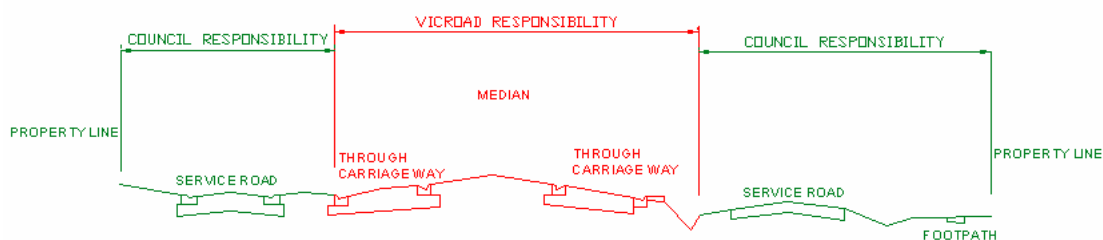
Figure 1 - Typical VicRoads Declared Main Road
